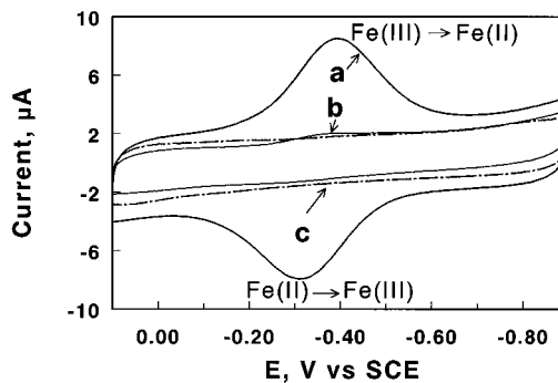
FIGURE 2. Cyclic voltammograms on basal plane PG electrodes at 100 \text{mV s}^{-1} in pH 7 buffer + 0.1 M KCl: (a) substrate-free cyt P450 cam –DMPC film in oxygen-free buffer containing no enzyme; (b) bare electrode in oxygen-free buffer containing 40 \mu\text{M} cyt P450 cam ; (c) DMPC film in oxygen-free buffer containing no enzyme. Adapted with permission from ref 25. Copyright 1997 Royal Society of Chemistry.
